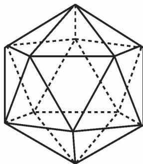
icosahedron
