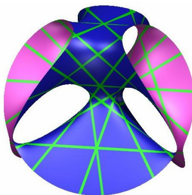
27 lines of cubic surface
